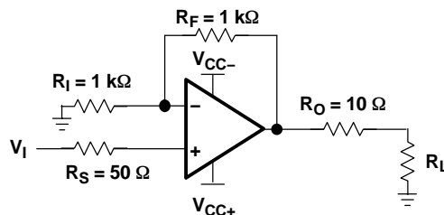
Figure 24. Single-Ended Input With a Noninverting Gain of 2 V/V
